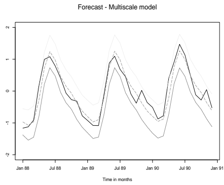
Fig. 8. Fraser river. Observed flow (solid), forecast (dashed) and predictive interval (dotted) for the years 1988, 1989 and 1990 by month.
