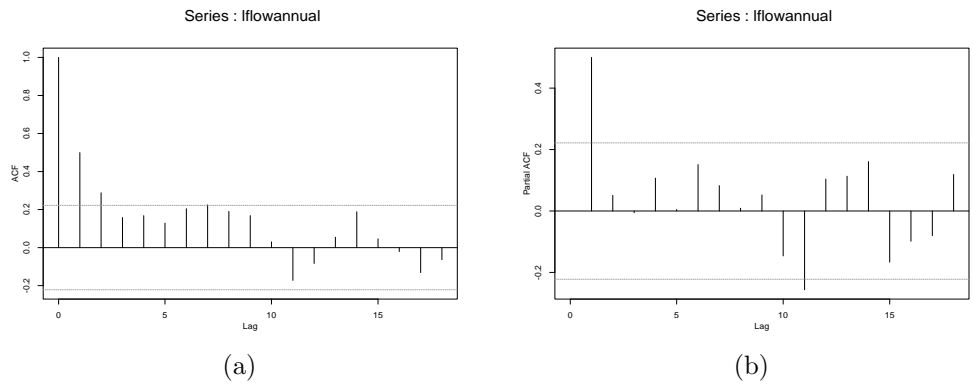
Fig. 3. Fraser river. (a) Autocorrelation and (b) partial autocorrelation functions of the annual series.
