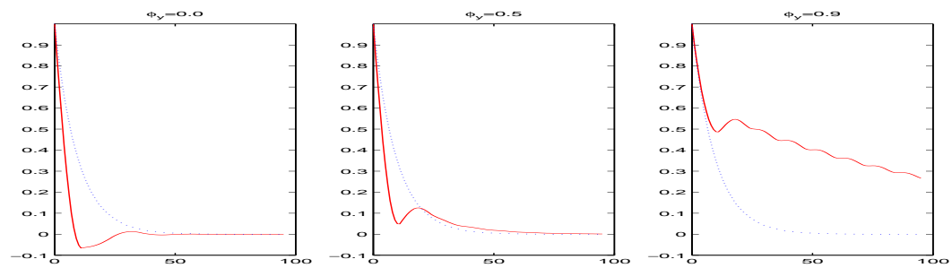
Fig. 4. AR(1) building blocks. Autocorrelation functions varying \phi_y (the autoregressive coefficient on the coarse scale). Parameters kept constant: \phi_x = 0.9 , \sigma_x^2 = 1 , \sigma_y^2 = 1 , \lambda = 0.1 and m = 12 . HRM (dashed line); AR(1) (dotted line).
