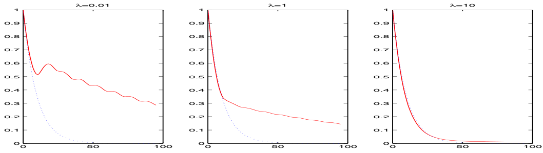
Fig. 5. AR(1) building blocks. Autocorrelation functions varying \lambda (the lack of agreement between coarse and fine levels). Parameters kept constant: \phi_x = 0.9 , \sigma_x^2 = 1 , \phi_y = 0.9 , \sigma_y^2 = 1 and m = 12 . HRM (dashed line); AR(1) (dotted line).
