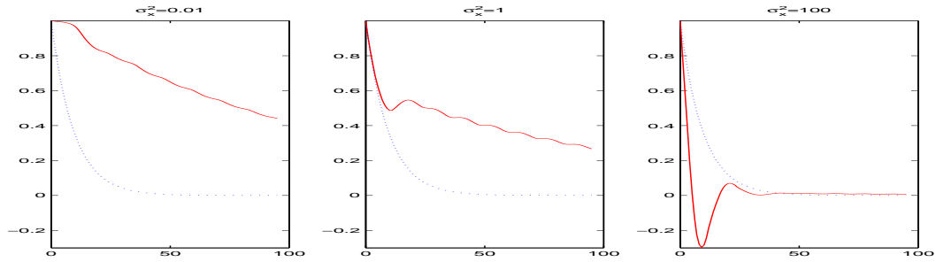
Fig. 7. AR(1) building blocks. Autocorrelation functions varying \sigma_x^2 (the variance of the error on the fine scale). Parameters kept constant: \phi_x = 0.9 , \phi_y = 0.9 , \sigma_y^2 = 1 , \lambda = 0.1 and m = 12 . HRM (dashed line); AR(1) (dotted line).
