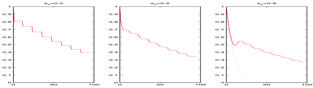
Fig. 6. AR(1) building blocks. Autocorrelation functions varying \phi_x (the autoregressive coefficient on the fine scale). Parameters kept constant: \sigma_x^2 = 1 , \phi_y = 0.9 , \sigma_y^2 = 1 , \lambda = 0.1 and m = 12 . HRM (dashed line); AR(1) (dotted line).
