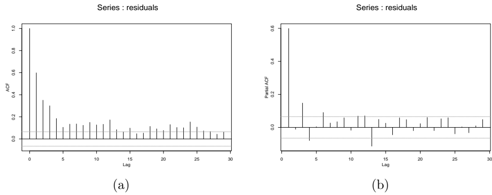
Fig. 2. Fraser river. (a) Autocorrelation and (b) partial autocorrelation functions of monthly residuals, suggesting a long memory process.
