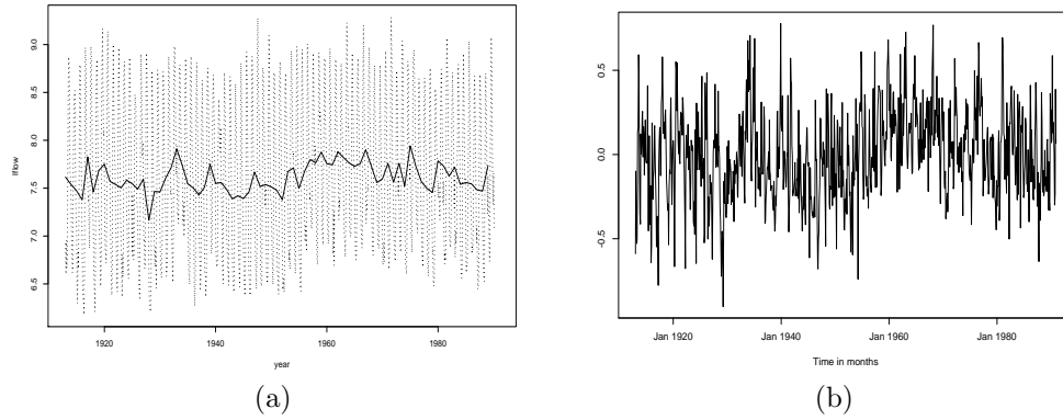
Fig. 1. Fraser River. (a) Log of the mean monthly flows (dotted) and annual averages (solid). (b) Monthly residuals after extracting the seasonality and the mean.
